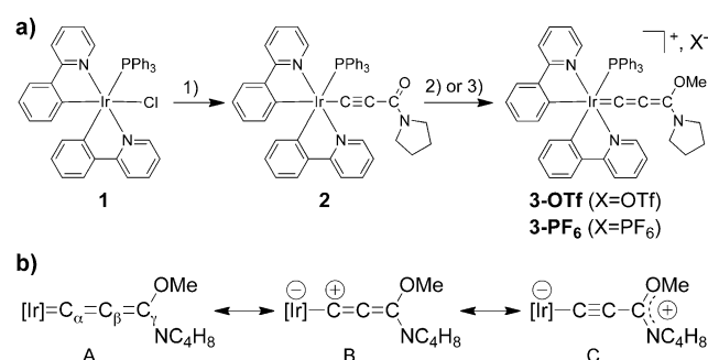
Scheme 1. a) Synthesis of alkynyl and allenylidene complexes. Reagents: 1) Ag-C\equiv C-C(=O)N(CH_2)_4 , 2) MeOTf , 3) MeOTf then KPF_6 ; b) resonance forms of allenylidene complexes.
